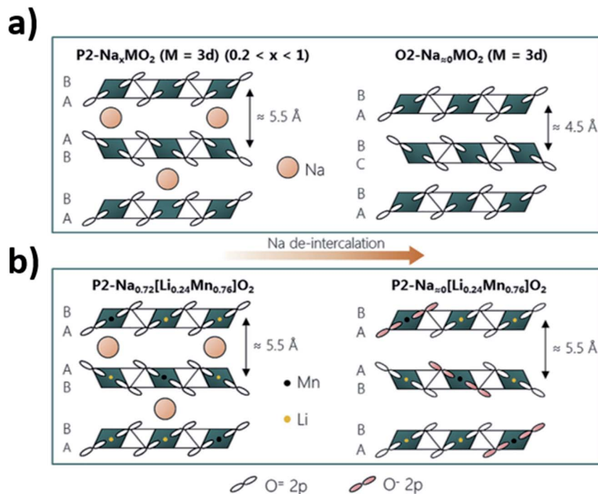
Fig. 13 Comparison of the structural changes that may take place upon extraction of sodium ions from (a) P2-type layered oxides that do not display oxygen redox activity and (b) the P2- Na_{0.72}[Li_{0.24}Mn_{0.76}]O_2 phase for which oxygen oxidation (highlighted in pink) partakes in the charge compensation mechanism. Reproduced with permission from ref. 115.
