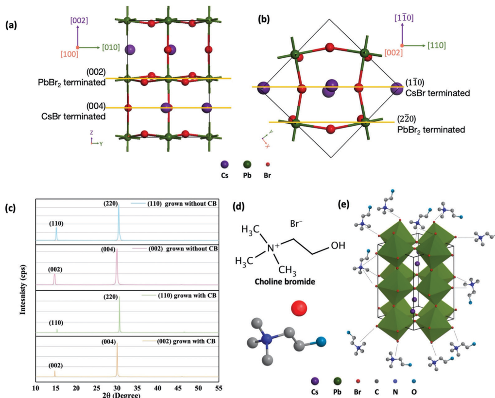
Fig. 2 (a) Side view of the orthorhombic \text{CsPbBr}_3 unit cell structure. The yellow lines indicate (002) and (004) plane. (b) Top view of the unit cell structure. The yellow lines indicate (1\bar{1}0) and (2\bar{2}0) plane. (c) XRD pattern of \text{CsPbBr}_3 single crystal grown with and without CB. (d) Molecular structure of choline bromide (CB). (e) Schematic illustration of CB assisted \text{CsPbBr}_3 single crystal growth.
