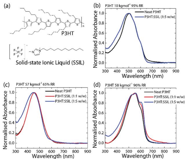
Fig. 1 (a) Chemical structure of the conjugated polymer P3HT and the solid state ionic liquid [C_{12}C_{12}IM^+][PF_6^-] (SSIL). Normalised absorbance spectra of P3HT neat, 1:1 and 1:5 for (b) low M_w and high RR, (c) high M_w and low RR and (d) high M_w and RR P3HT blends.
