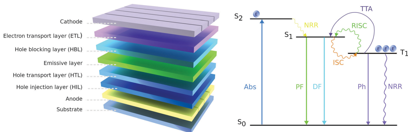
Fig. 15 The structure of OLED (left); simplified Jablonski diagram representing emission process in the OLED (right), where E – exciton, Abs – absorption, PF – prompt fluorescence, DF – delayed fluorescence, Ph – phosphorescence, NRR – non-radiative relaxation, ISC – intersystem crossing, RISC – reverse intersystem crossing, TTA – triplet-triplet annihilation.
