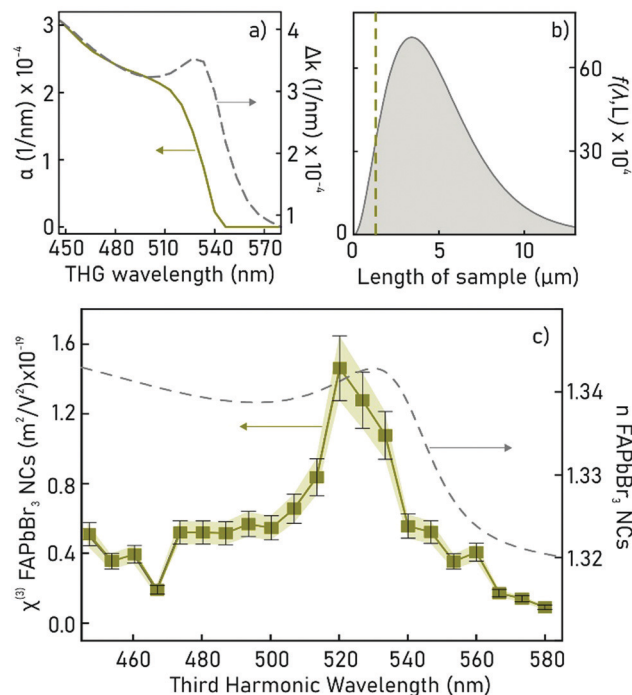
Fig. 4 Extraction of third-order nonlinear susceptibility ( \chi^{(3)NC} ) of a ncFAPbBr 3 @SiO 2 film. (a) Spectral behaviour of the absorption coefficient of the third harmonic wave and the phase mismatch between the fundamental and the third harmonic waves. (b) Calculated f(\lambda, L) , which is proportional to third harmonic intensity, versus ncFAPbBr 3 @SiO 2 film thickness ( \lambda_1 = 1560 nm, \lambda_3 = 520 nm). The vertical dashed line indicates the actual thickness of the composite film (1300 nm). (c) Spectral dependence of both the estimated third order nonlinear susceptibility of the FAPbBr 3 nanocrystals after volume correction and the linear refractive index of the composite (dashed line).
