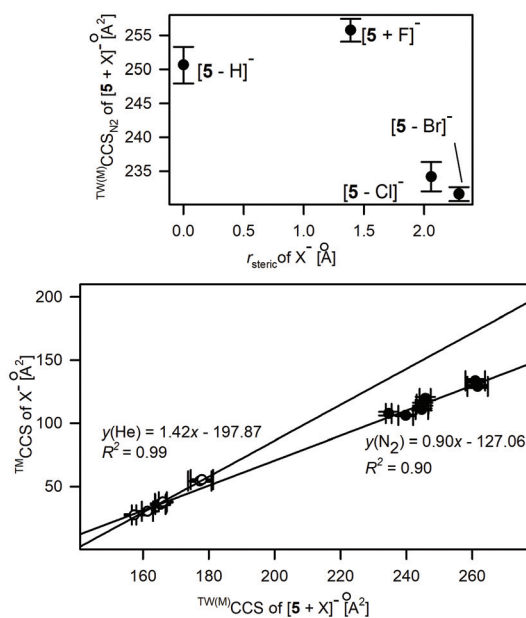
Fig. 7 Relationship between X^- anionic radius, r_{\text{steric}} (upper panel) or ^{TM}CCS values of polyatomic X^- and the experimental CCS values of [5 + X]^- .
