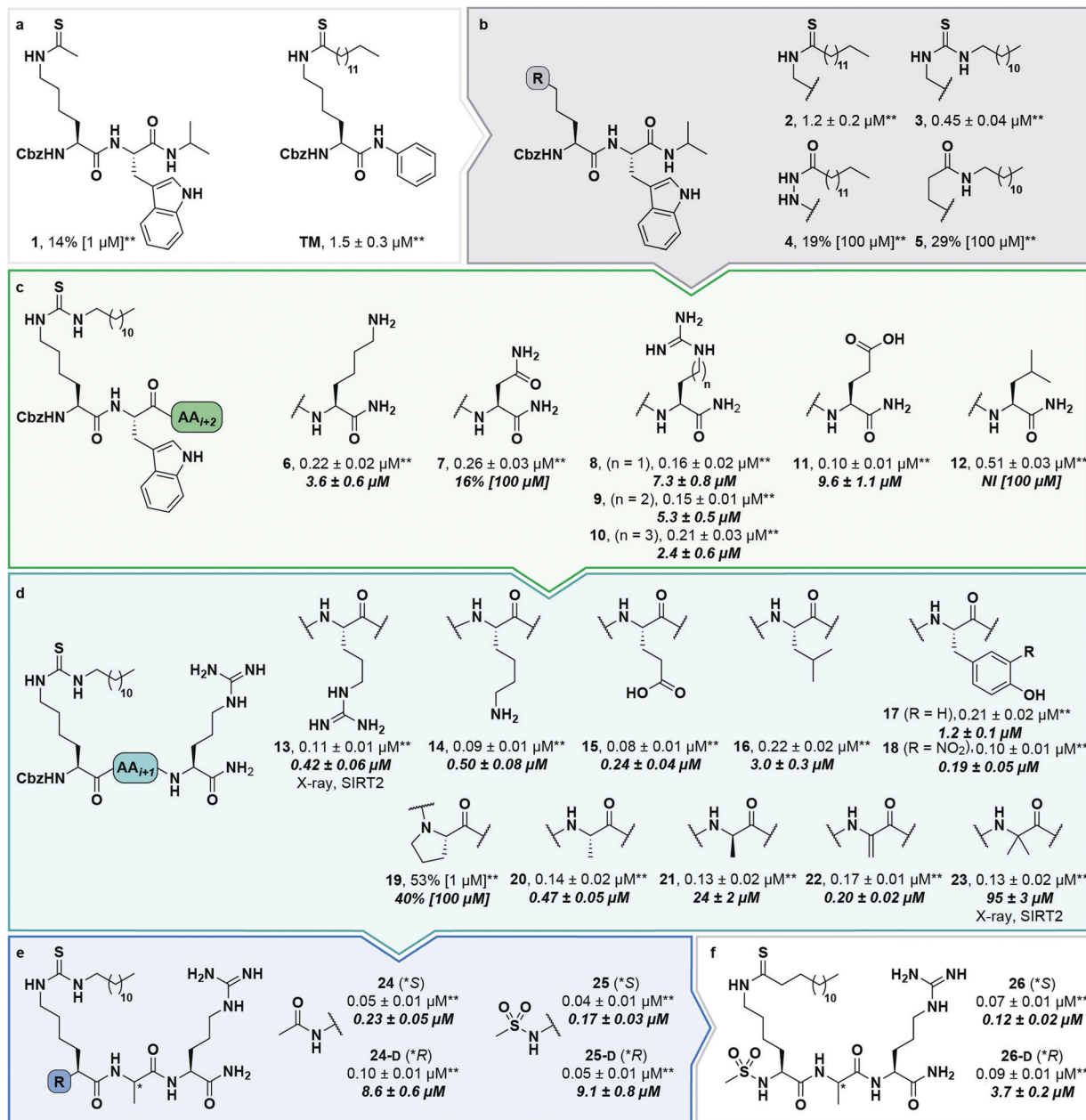
Scheme 1 Structure–activity relationship of SIRT2 inhibitors. Potencies for inhibition of the deacylase activity of recombinant SIRT2 (100 nM) against QPKKac (shown with asterisks**) or ETKmyr (shown in bold/italics) as substrate (50 \mu\text{M} ) are given as mean \text{IC}_{50} values \pm standard deviation (SD) or %inhibition. (a) Lead compounds. (b) Amide isosteres. (c) Optimization of position i + 2 . (d) Optimization of position i + 1 . (e) Optimization of N-terminal group. (f) Final inhibitors. Data are based on two individual experiments performed in duplicate. See the ESI† (Scheme S1, Fig. S1–S3 and Table S2) for dose–response curves and selectivity profiling of additional inhibitors (S17–S23) against SIRT1–3. *A single asterisk denotes a stereogenic center.
