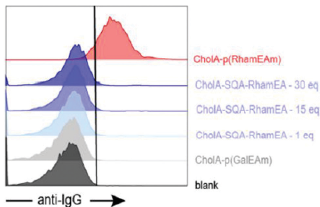
Fig. 5 Antibody recruitment with polymers (ChoIA-p(RhamEAm) versus different concentrations of a single rhamnose moiety linked to ChoIA (ChoIA-SQA-Rham), with ChoIA-p(GalEAm) used as the negative control (reproduced from ref. 12 with permission from American Chemical Society, copyright 2020).
