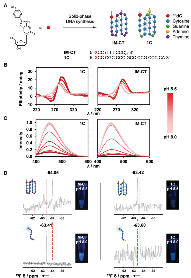
Fig. 2 Characterization of FPdC-containing i-motif structures. (A) I-Motif-forming DNA sequences, 1C and IM-CT, containing FPdC. (B) CD and (C) normalized fluorescence spectra of 1C and IM-CT with pH. (D) 19 F NMR spectra and images of 1C and IM-CT.
