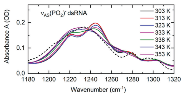
Fig. 13 Linear infrared absorption spectra of the \nu_{\text{AS}}(\text{PO}_2)^- stretching vibrations of (\text{AU})_{23} dsRNA in water at different sample temperatures (RNA concentration c(\text{RNA}) = 2.3 \text{ mM} ). In the temperature range 303–333 K, infrared spectra are shown in increments of 10 K. 5 K increments were employed above 333 K to highlight the major changes in the spectra around 338 K. Dashed line: infrared absorption of DNA oligomers at 303 K. The spectrum is scaled to the RNA peak absorption at 1230 \text{ cm}^{-1} ( T = 353 \text{ K} ). Adapted with permission from ref. 72. Copyright 2020 American Chemical Society.
