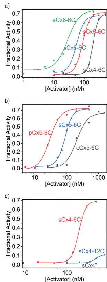
Fig. 3 Hill plots for (a) sCx4-6C , sCx5-6C , sCx6-6C , and sCx8-6C , (b) sCx5-6C , cCx5-6C , and pCx5-6C , and (c) sCx4 , sCx4-6C , and sCx4-12C for Arg9 transport activation. With the exception of sCx4 , data were fitted to the Hill equation.
