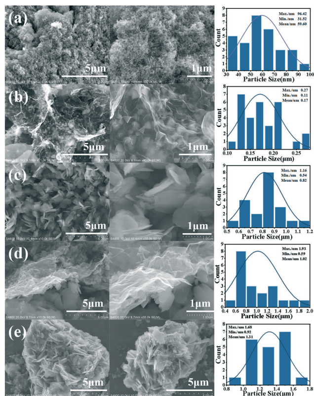
Fig. 2 SEM images and particle size distribution diagrams of pristine \text{Co}_3\text{O}_4 (a) and g\text{-Co(OH)}_2 with different hydrothermal reaction times: (b) 3 h; (c) 6 h; (d) 9 h and (e) 12 h.
