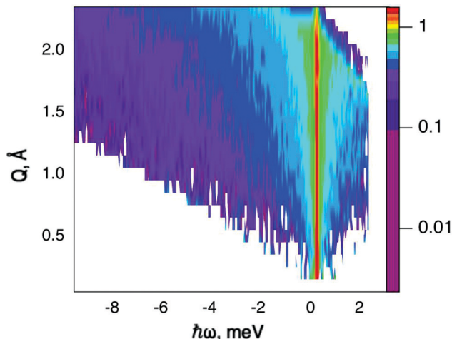
Fig. 2 Scattering function, S(\mathbf{Q}, \omega) , of hydrogen loaded MoS 2 single crystals, measured at 400 K with the sample's basal planes oriented parallel to the momentum transfer vector \mathbf{Q} . The plot uses a logarithmic intensity scale. Higher intensities are represented by red colour and lower intensities by blue. White area: no data, since it falls outside of the spectroscopic window.
