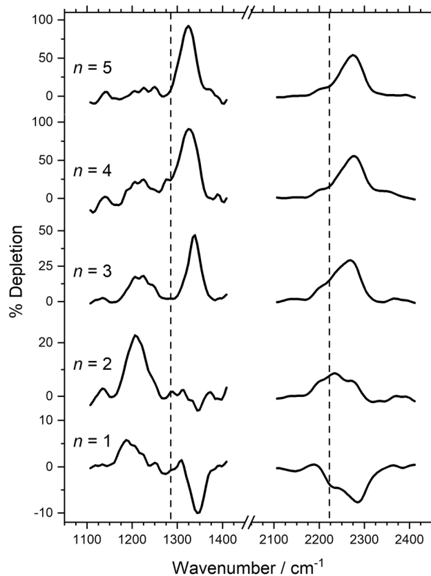
Fig. 6 IR-MPD depletion spectra of Co n (N 2 O) + ( n = 1-5 ) clusters in the N=O and N=N regions of N 2 O. The vertical dashed lines at 1285 and 2224 cm -1 indicate the wavenumber of the ν 1 (N=O) and ν 3 (N=N) modes in isolated N 2 O, respectively. 55
