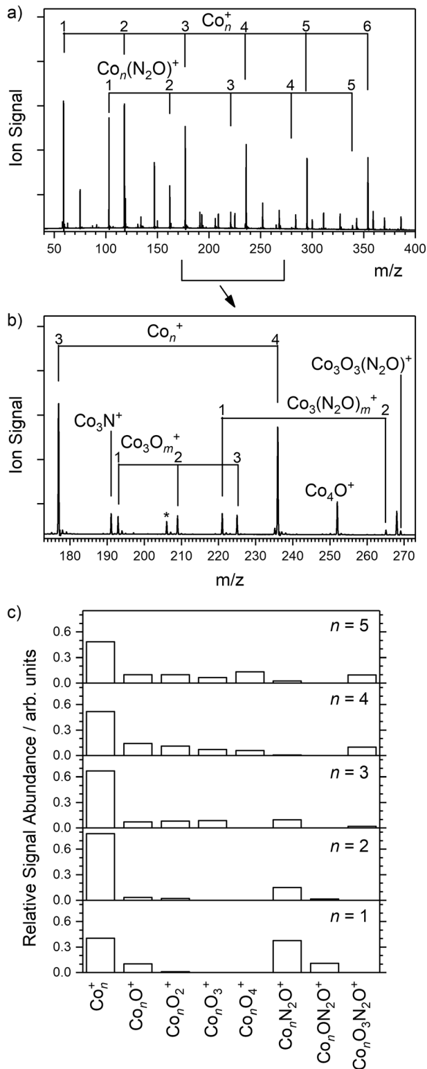
Fig. 5 (a and b) Mass spectrum of ions observed following ablation of a cobalt rod along with N 2 O added downstream in the cluster channel. For clarity, the mass signal for Co 2 (N 2 O) 2 + is marked with an asterisk (*). (c) Histogram showing relative abundance of major species observed relative to the naked Co n + mass signal. The larger clusters react readily with N 2 O forming simple oxides.
