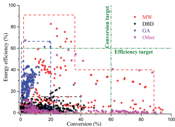
Fig. 6 CO 2 conversion and energy efficiency achieved in different plasma experiments. The data points represent the results. Black: labeled DBD: dielectric barrier discharge; Blue: labeled GA: gliding arc; Red: labeled MW: Microwave and radiofrequency plasma. Most data redrawn from ref. 20. To give an indication of the performance we have drawn green dash-dotted lines to represent an efficiency and a conversion target, both set at 60%. The conversion efficiency we took at 60% because several studies mentioned in the review show that this value can be obtained and exceeded; see also the discussion on page 5826 of ref. 20.
