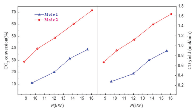
Fig. 14 \text{CO}_2 conversion and CO yield in triple flow experiments operated in two different modes discussed in the text.
