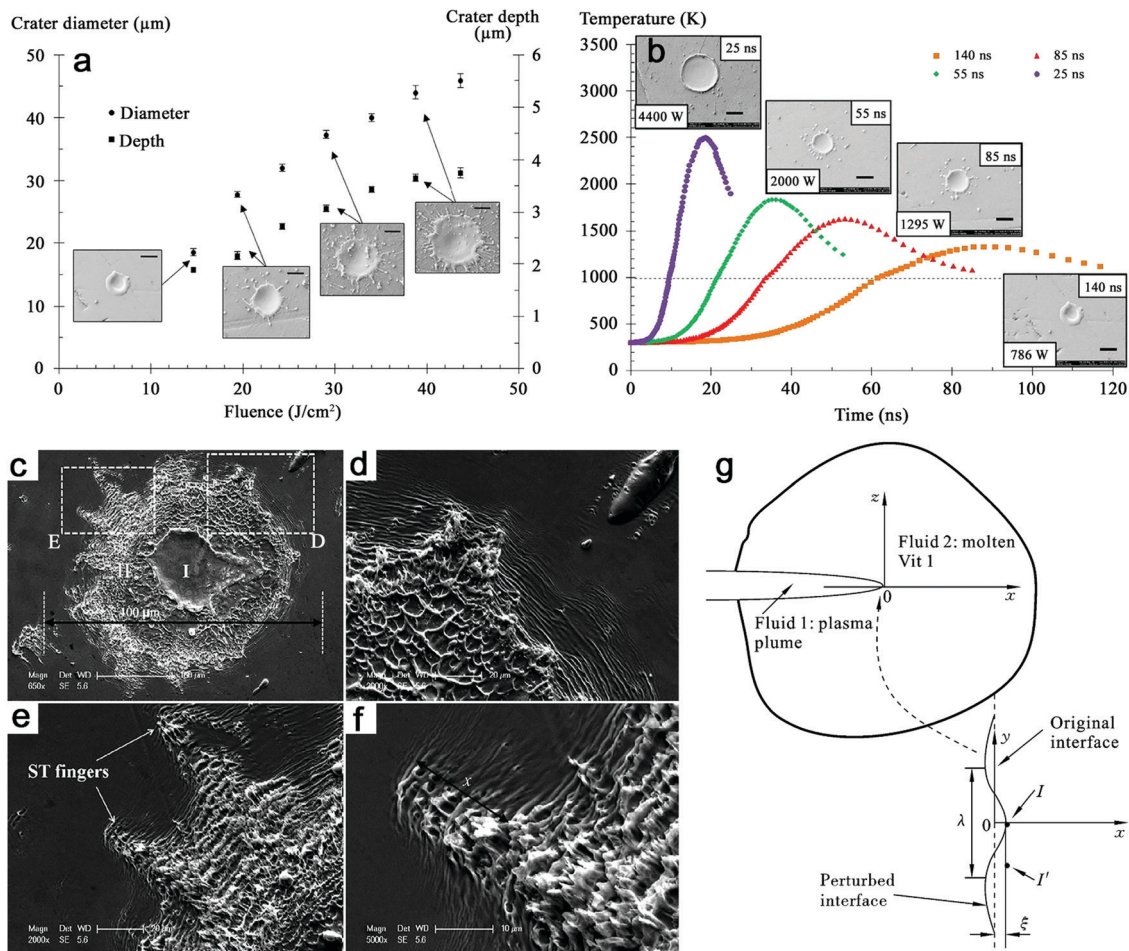
Fig. 12 Surface characteristics of Zr-based MG after laser ablation. (a) Crater diameter and depth as a function of the fluence for a 140 ns pulse. Scale bars in SEM images: 20 µm. (b) Predicted temporal temperature variation at a fluence of 14 J cm -2 for pulse durations of 140 ns, 85 ns, 55 ns, and 25 ns. Scale bars in SEM images: 20 µm. Reproduced with permission from ref. 206. (c–f) Surface morphologies of ns-laser ablation of Vitreloy 1 in water showing surface ripples and Saffman–Taylor fingering. (g) Development of Saffman–Taylor fingering instability at a meniscus-shaped interface between the plasma plume and the molten Vitreloy 1. Adapted with permission from ref. 207.
