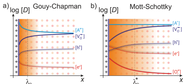
Fig. 5 Schematic illustration of the space-charge region for (a) Gouy-Chapman and (b) Mott-Schottky case. Adapted from ref. 60 with permission.
