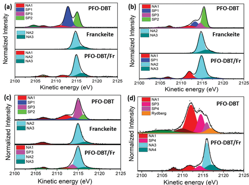
Fig. 4 S K- L_{2,3}L_{2,3} RAS spectra of PFO-DBT, exfoliated franckeite and PFO-DBT/Fr thin films collected at the photon energies of (a) 2471.8 eV (B1), (b) 2472.5 eV (T1), (c) 2473.5 eV (B2), and (d) 2474.5 eV (T2).
