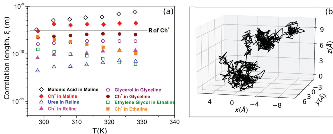
Fig. 6 (a) Correlation length of different species in maline, reline, glycine and ethaline calculated from eqn (5) using the diffusion constant obtained from PFG-NMR (adapted from ref. 74). (b) MD simulation trajectory of acetamide molecules in DES (acetamide + lithium perchlorate, 78 : 22), showing both long-range jumps and the localised diffusion within the cages (adapted from ref. 20).
