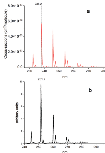
Fig. 15 Comparison of an A ^1\Pi-X^1\Sigma^+ simulated emission spectrum (panel a) with that recorded by Moeller and Silvers. 13 (panel b). The number at the top indicates the centre of the peak. The spectrum was simulated at T_{\text{rot}} = 500 K (rotational) and T_{\text{vib}} = 1200 K (vibrational) temperatures with a Gaussian profile of HWHM = 100 \text{cm}^{-1} .
