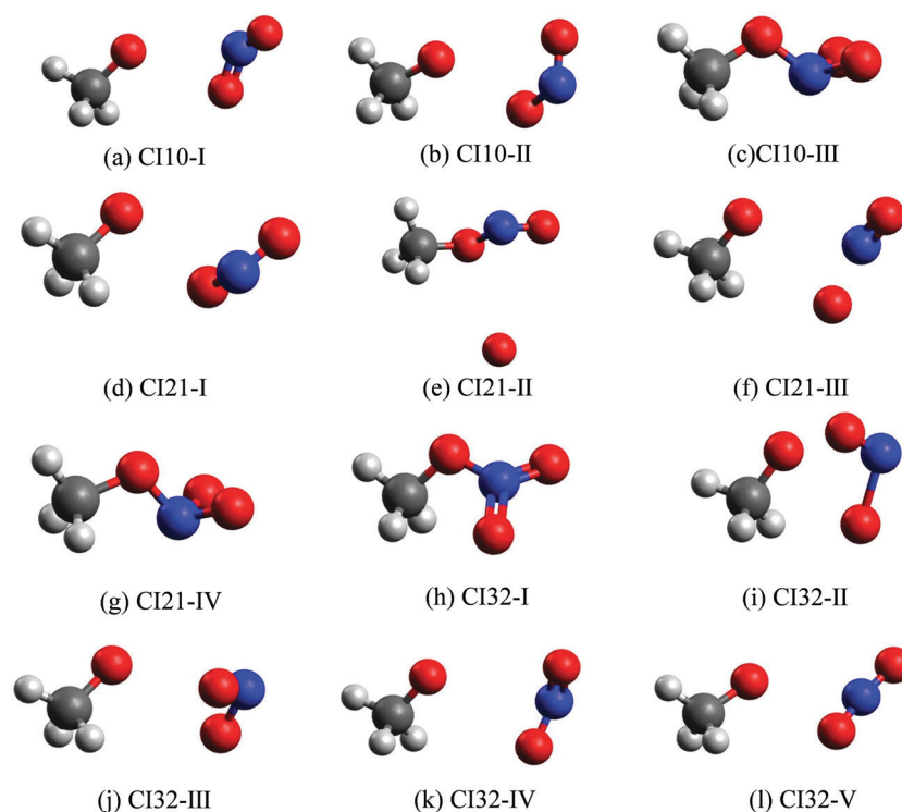
Fig. 3 The MECIs optimized at the SA(4)-CASSCF(12,9)/cc-pVDZ level: (a)–(c): S_1 – S_0 CIs; (d)–(g): S_2 – S_1 CIs; (h)–(l): S_3 – S_2 CIs.
