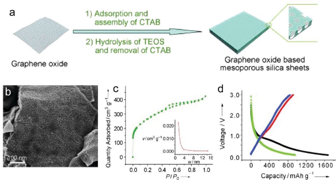
Fig. 14 (a) Schematic of the formation process for graphene oxide based mesoporous silica sheets. (b) SEM and (c) nitrogen adsorption/desorption isotherm of the obtained graphene-based mesoporous nanosheets. (d) First and second cycles of galvanostatic discharge/charge curves of the graphene-based mesoporous nanosheets. Reproduced from ref. 241 with permission from Wiley-VCH.
