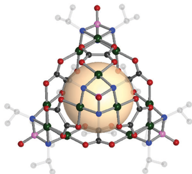
Fig. 10 Structural illustration of [(\text{Pd}_3[(\text{N}^i\text{Pr})_3\text{PO})_4(\text{A19})_6)]_6 . 60
