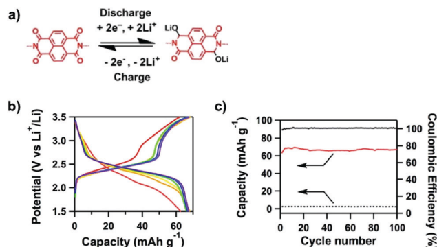
Fig. 68 (a) Electrochemical redox reaction of a naphthalene diimide unit. (b) Discharge–charge curves of D_{TP}\text{-}A_{NDI}\text{-COF@CNTs} upon 100 cycles at a rate of 2.4C (red, 1st cycle; orange, 10th cycle; yellow, 20th cycle; green, 50th cycle; blue, 80th cycle; and purple, 100th cycle). (c) Capacities of D_{TP}\text{-}A_{NDI}\text{-COF@CNTs} (red line) and CNT (dotted black line) batteries and coulombic efficiencies of D_{TP}\text{-}A_{NDI}\text{-COF@CNTs} for 100 cycles (black line). Adapted with permission from ref. 324, Copyright 2015 Springer Nature.
