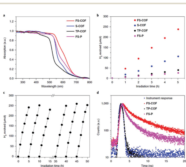
Fig. 40 (a) Optical absorption and (b) photocatalytic \text{H}_2 production as a function of time of the FS-COF, S-COF, TP-COF (reference without sulfone moiety) and the FS-P (analogous amorphous polymer). (c) Stability tests of the catalytic activity of FS-COF and (d) time-correlated single photon counting traces of the FS-COF, reference TP-COF and amorphous FS-P. Reproduced with permission. 207 Copyright 2018, Nature Publishing Group.
