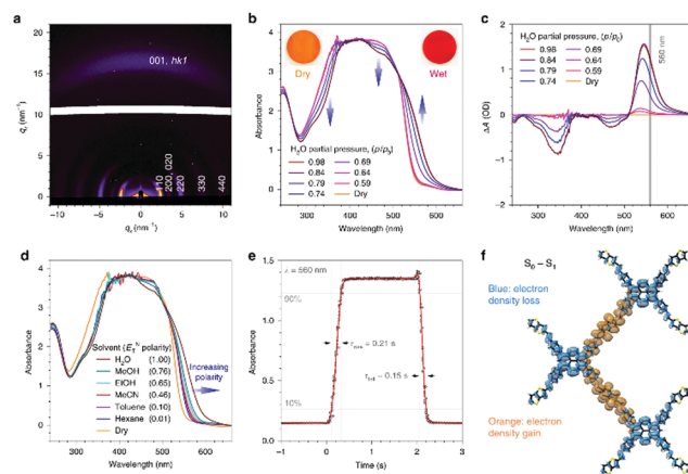
Fig. 43 (a) GIWAXS pattern of oriented Py-TT COF film on sapphire. (b) UV-Vis absorption of COF film at different moisture contents. (c) Humidity-induced absorbance changes. (d) UV-Vis absorption of COF film in saturated solvent atmospheres. (e) Solvatochromic response of COF film to changes from dry to H 2 O-saturated N 2 -streams and back. (f) TD-DFT calculated electron density difference upon the one-electron excitation from ground state to the first singlet excited state showing a distinct charge-transfer character. Reproduced with permission. 19 Copyright 2018, Nature Publishing Group.
