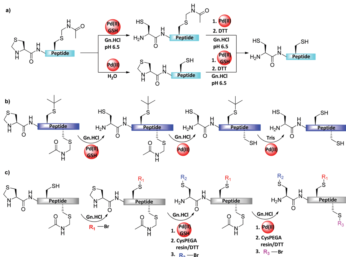
Fig. 17 Cys deprotection on demand: (a) \text{Pd(II)} -mediated selective removal of Acm and Thz groups, (b) \text{Pd(II)} -mediated selective removal of Acm, Thz, and t-butyl groups, (c) \text{Pd(II)} -mediated site-specific and differential modification of a peptide.
