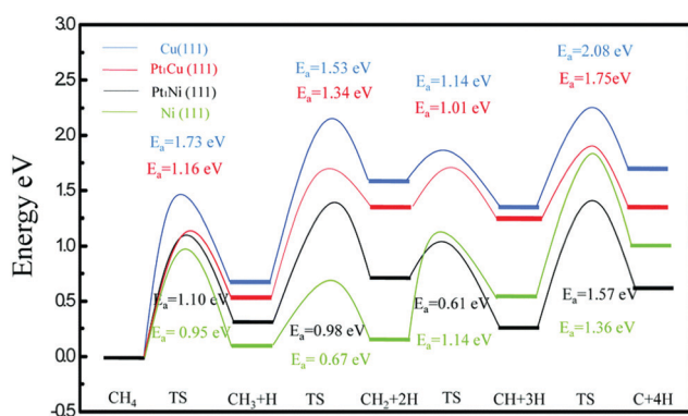
Fig. 17 Comparison of methane dissociation reaction pathways on \text{Pt}_1\text{Cu}(111) and \text{Pt}_1\text{Ni}(111) surfaces. 231 Reproduced from ref. 231 with permission from the Centre National de la Recherche Scientifique (CNRS) and the Royal Society of Chemistry, copyright 2020.
