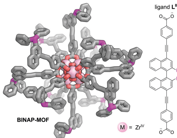
Fig. 11 The \text{Zr}_6\text{O}_4(\text{OH})_4(\text{O}_2\text{CR})_{12} SBUs bound by 12 \text{L}^8 bridging ligands which bridge adjacent clusters to form BINAP-MOF . Post-metalation with [\text{Rh}(\text{nbd})_2](\text{BF}_4) yields BINAP-MOF-Rh , which acts as a catalyst for the conjugate addition of arylboronic acids to 2-cyclohexanone. 50 Hydrogen atoms omitted for clarity. Colours: C grey, O red, P magenta, Zr light pink (shown as spheres).
