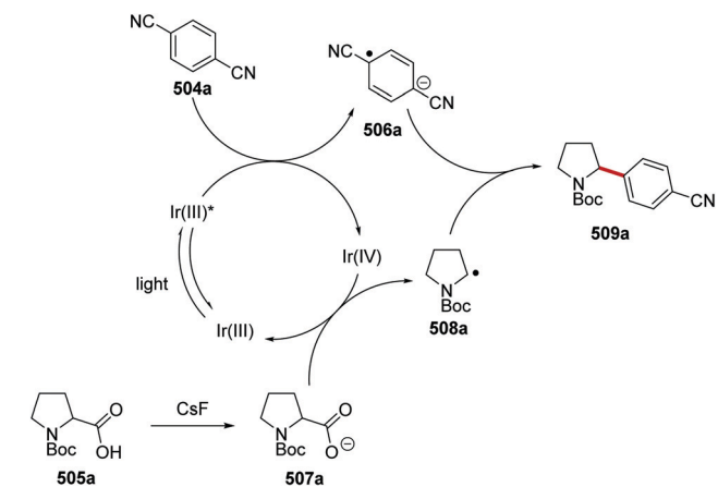
Scheme 145 Radical coupling between benzonitrile 504a and carboxylic acid radical precursor 505a .
