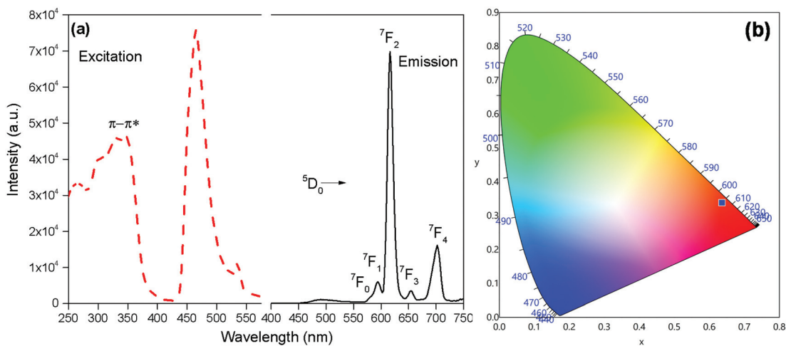
Fig. 4 (a) Excitation (broken line) and emission (solid line) spectra ( \lambda_{\text{ex}} = 345 \text{ nm} ) (b) CIE-1931 chromaticity diagram demonstrating the calculated colour coordinate ( x, y ) values for [\text{Eu}(\text{btfa})_3\mathbf{1c}] in DCM at RT.
