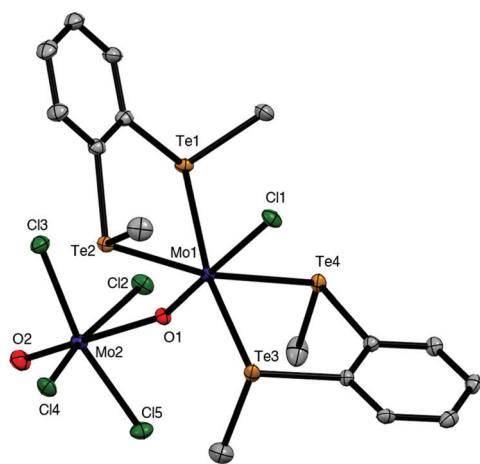
Fig. 5 Crystal structure of [\text{MoCl}\{o\text{-C}_6\text{H}_4(\text{TeMe})_2\}_2(\mu\text{-O})\text{MoOCl}_4] \cdot \text{CH}_2\text{Cl}_2 showing the atom numbering scheme. Ellipsoids are shown at 50% probability and hydrogen atoms and solvent are omitted for clarity. Selected bond lengths (Å) and angles ( ^\circ ): \text{Mo1}-\text{Cl1} = 2.4486(7) , \text{Mo2}-\text{Cl2} = 2.3640(7) , \text{Mo2}-\text{Cl2} = 2.3930(7) , \text{Mo1}-\text{Te1} = 2.7432(3) , \text{Mo1}-\text{Te1} = 2.7822(3) , \text{Mo1}-\text{O1} = 1.704(2) , \text{Mo2}-\text{O1} = 2.370(2) , \text{Mo2}-\text{O2} = 1.655(2) , \text{O2}-\text{Mo2}-\text{Cl2} = 78.4(1) , \text{O2}-\text{Mo2}-\text{Cl2} = 82.2(1) , \text{Te}-\text{Mo1}-\text{Te}_{(\text{chelate})} = 85.316(8) , 86.185(8) , \text{Te1} = 4-\text{Mo1}-\text{Cl1} = 79.647(18) , 89.939(18) , \text{Cl1}-\text{Mo1}-\text{O1} = 177.91(7) , \text{Mo1}-\text{O1}-\text{Mo2} = 159.631(11) .
