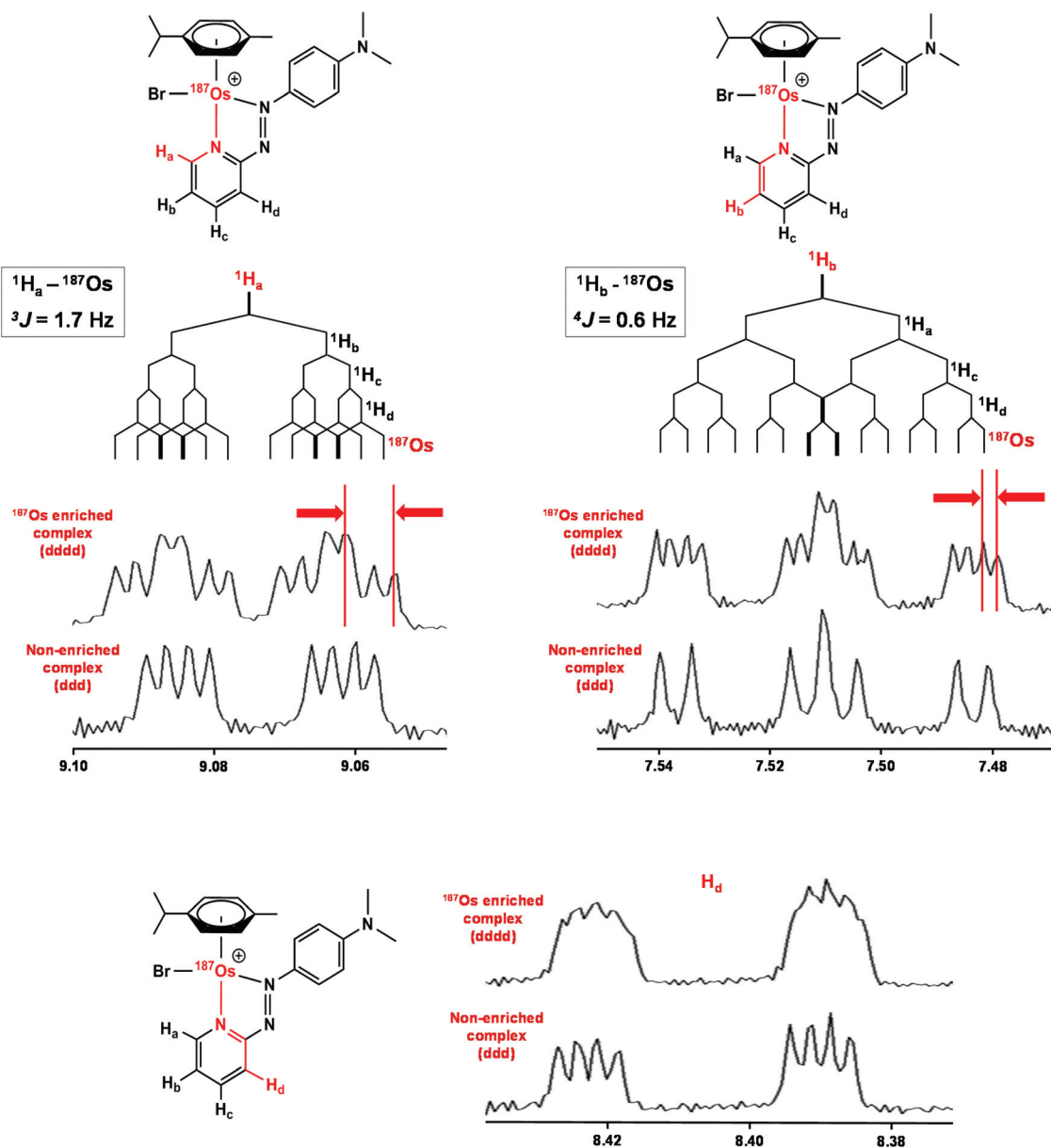
Fig. 4 ^1\text{H} NMR (250 MHz) spectra of ^{187}\text{Os} - 1 compared to natural abundance 1 , with expansions of the resonances for ^1H_a , ^1H_b , and ^1H_d illustrating their couplings to other protons and ^{187}\text{Os} . Samples were prepared in \text{MeCN}-d_3 .
