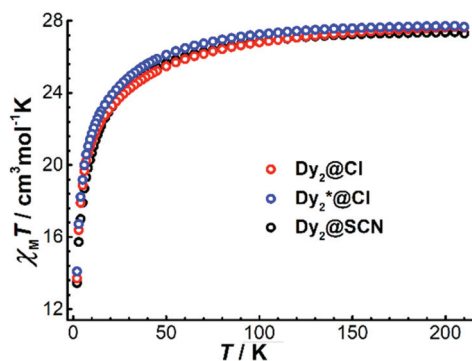
Fig. 5 Temperature dependence of the product \chi_M T for Dy 2 Cl , Dy 2 * Cl , and Dy 2 NCS at 5000 Oe between 2 and 210 K.
