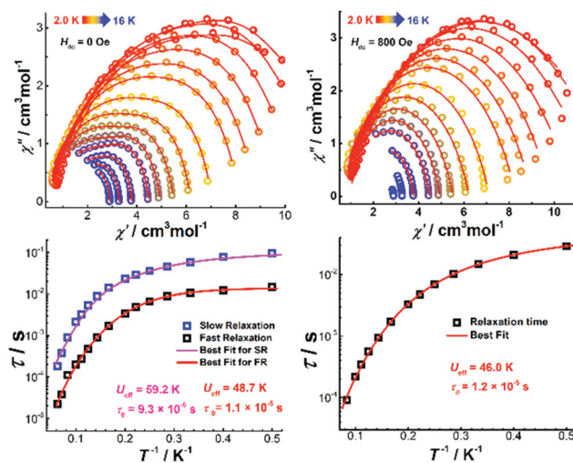
Fig. 7 The Cole–Cole diagrams (top) and \tau vs. T^{-1} plots (bottom) under zero (left) and 800 Oe (right) dc field for Dy 4 . The solid lines indicate the best fits.
