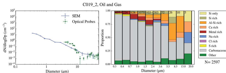
Fig. 3 Aerosol size distribution and size-resolved composition of the samples collected on 2017/07/11 (oil and gas). PCASP data not available for this flight due to technical problems.
