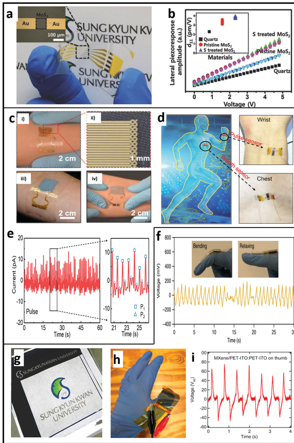
Fig. 10 Small-scale PENG and TENG demonstrators enabled by GRM. (a) Photograph of the MoS 2 nanosheet-based flexible piezoelectric device on a PET substrate. (b) Lateral piezoelectric response of the pristine monolayer MoS 2 , S-treated monolayer MoS 2 , and \alpha -Quartz, using lateral Piezoresponse force microscopy methods. (Panels a and b are reproduced with permission. 308 Copyright 2018 WILEY-VCH Verlag GmbH & Co. KGaA, Weinheim) (c) flexible PENG for wearable applications. Panel (i): optical image of the in-plane electrodes for piezoelectric thin films with PI supporting layer and PDMS substrate. Panel (ii): enlarged optical image of the electrode pattern. Panels (iii) and (iv): optical images of the rubbery piezoelectric electronics attached on the surface of forearm, and deformations together with skin. (Reproduced with permission. 310 Copyright 2019 WILEY-VCH Verlag GmbH & Co. KGaA, Weinheim) (d) realtime monitoring of physiological signals (left). (e) Real-time monitoring of arterial pulse signals (panels d and e Reproduced with permission. 26 Copyright 2019 American Chemical Society). (f) Output measurement in a practical wearable device application based on SnS PENG. (Reproduced with permission. 314 Copyright 2020 Nature.) (g) Driving a commercial LCD using graphene enabled TENG. The left panel presents the OFF state, and the right panel presents the ON state of the LCD units. (Reproduced with permission. 126 Copyright 2014 WILEY-VCH Verlag GmbH & Co. KGaA, Weinheim.) (h) MXene-based flexible TENG mounted on a thumb for harvesting energy from simple human muscle movements. (i) V_{oc} varying between -40 and 70 V was generated by the TENG mounted on the thumb. (Panel h and I reproduced with permission. 316 Copyright 2018 Elsevier.)
