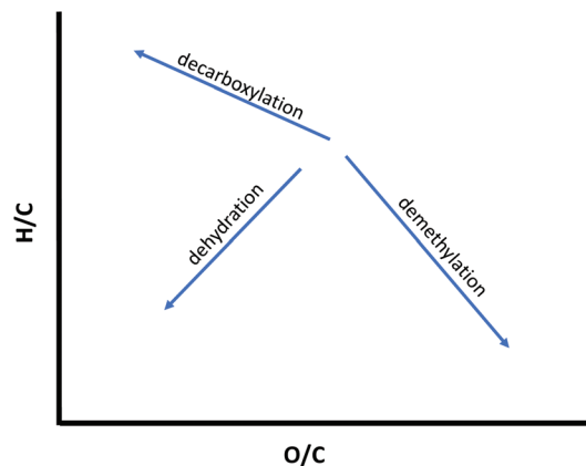
Fig. 3 Van Krevelen diagram for reaction pathways during the microwave-assisted hydrothermal processing of biomass.
