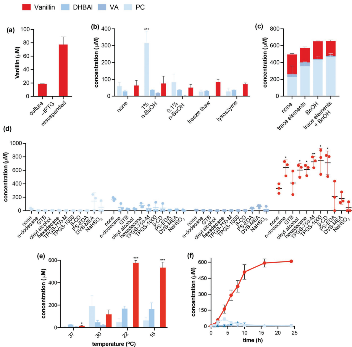
Fig. 3 Optimisation of vanillin pathway expression and biotransformation conditions. (a) Comparison between fermentation and resuspended whole cells (conditions: 5 mM TA added to 10 mL fermentation reactions at time of induction, incubated at 30 °C for 24 hours). (b) Effect of cell membrane permeabilisation (conditions: 5 mM TA, 30 °C, 24 hours). (c) Effect of addition of trace elements and benzyl alcohol (BnOH) to expression medium (conditions: 5 mM TA, 30 °C, 24 hours). (d) Effect of in situ product removal (ISPR) (conditions: 1 mM TA, 22 °C, 24 hours). (e) Effect of biotransformation temperature (conditions: 5 mM TA, 24 hours). (f) Time course of TA conversion under optimised conditions (1 mM TA, 22 °C, 20%v/v oleyl alcohol (OA)). GTB: Glycerol tributyrate; TPGS: DL - \alpha -tocopherol methoxypolyethylene glycol succinate; \beta -CD: \beta -cyclodextrin; PS-EDA: ethylenediamine, polymer bound, 1% cross-linked (1%w/v loading); DVB-MEA: mercaptoethylamine, polymer bound, 1% cross-linked with divinylbenzene (1%w/v loading). * P < 0.05 , ** P < 0.005 , *** P < 0.0005 (Welch's T -test).
