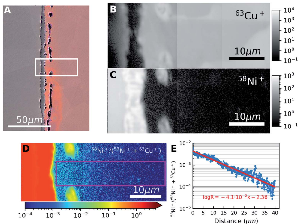
Fig. 2 (A) Same as Fig. 1(A) but with the area used for SIMS acquisition outlined. (B and C) Montage SIMS images of 63 Cu + and 58 Ni + obtained by post-acquisition alignment of three overlapping images placed side-by-side with logarithmic intensity scales. (D) SIMS ratio image 58 Ni + / (58 Ni + + 63 Cu + ) obtained from (B and C). The colour bar indicates SIMS ratio values. (E) SIMS ratio plot (from D) obtained by vertically averaging the values in the pink rectangle in (D). The red line shows a linear fit of the data in the semi-log plot.
