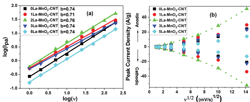
Fig. 8 \log(I_{pa}) vs. \log(v) plot (a); and I_{pc} vs. v^{1/2} plot (b) of all the samples.
