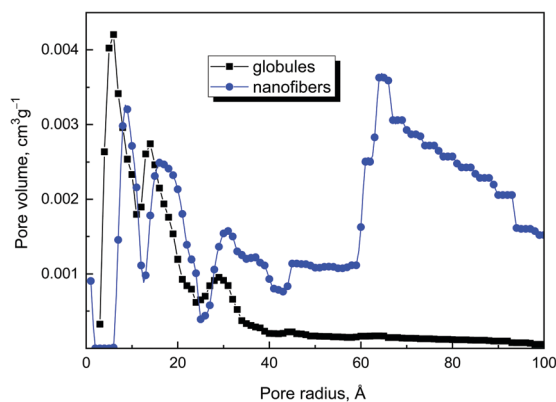
Fig. 11 Pore size distribution of original globules and nanofibers.
