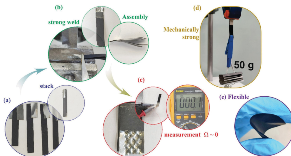
Fig. 6 Four steps for welding buckypapers: (a) stacking, (b) welding, (c) measuring the electric contact, and (d) evaluation of the mechanical robustness, showing (e) the flexible material.
