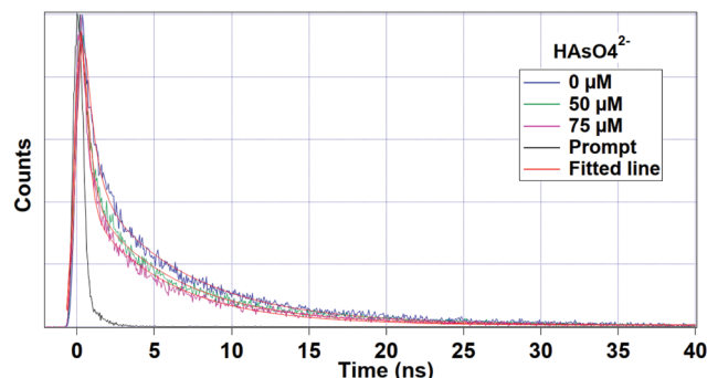
Fig. 6 Luminescence lifetime decay profile and the corresponding fitted line of 1a before and after the addition of \text{HAsO}_4^{2-} anions. The final concentration of \text{HAsO}_4^{2-} ions in the medium is indicated in the legend. The instrument response function (prompt) is also shown. Here, \lambda_{\text{ex}} = 280 \text{ nm} and \lambda_{\text{em}} = 420 \text{ nm} (ligand centre emission) were set during the experiment.
