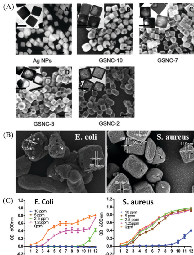
Fig. 10 (A) SEM and TEM (inset) images of Au–Ag nanocages (scale bar is 50 nm) produced by reacting Ag nanocubes with varying amount of HAuCl 4 to tailor different molar ratios of Ag/Au. (B) SEM images of E. coli and S. aureus to indicate cavities on the membrane, which matches with the Au–Ag nanocages, and (C) the corresponding E. coli and S. aureus growth curve with different concentrations of Au–Ag nanocages. Reproduced from ref. 172 with permission from the Royal Society of Chemistry.
