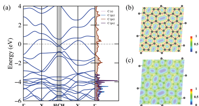
Fig. 4 (a) Electronic band structure and projected density of states of C_{5678} . Fermi level was set to zero. (b) ELF of C_{5678} with slices (b) crossing the structure plane and (c) 1 \text{ \AA} above the structure plane.
