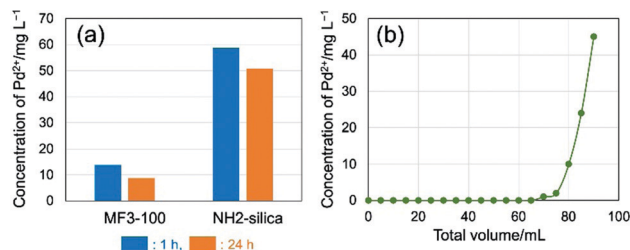
Fig. 5 (a) Concentrations of \text{Pd}^{2+} in the batch adsorption tests using granulated MF3-100 and aminopropyl-modified silica in 0.1 \text{ mol L}^{-1} HCl with 100 \text{ mg L}^{-1} \text{Pd}^{2+} for 1 and 24 h. (b) Change in the \text{Pd}^{2+} concentration with the total flowed volume in the flow adsorption test using granulated MF3-100.
