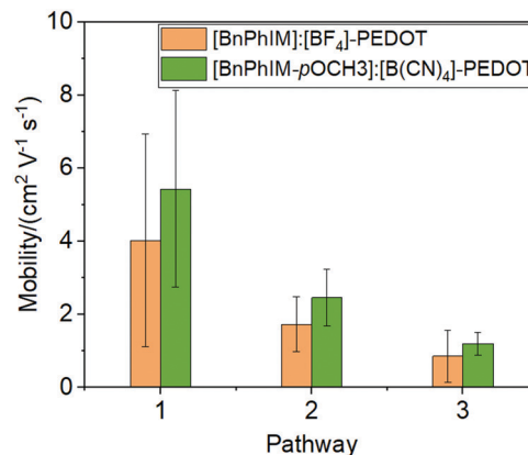
Fig. 9 A comparison of mobility in [BnPhIM]:[BF 4 ]-PEDOT and [BnPhIM- p OMe]:[B(CN) 4 ]-PEDOT.
