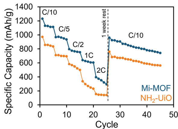
Fig. 5 Rate performance of Mi-UiO-66 (blue) and NH 2 -UiO-66 (orange) cells cycled at C/10, C/5, C/2, 1C and 2C.
