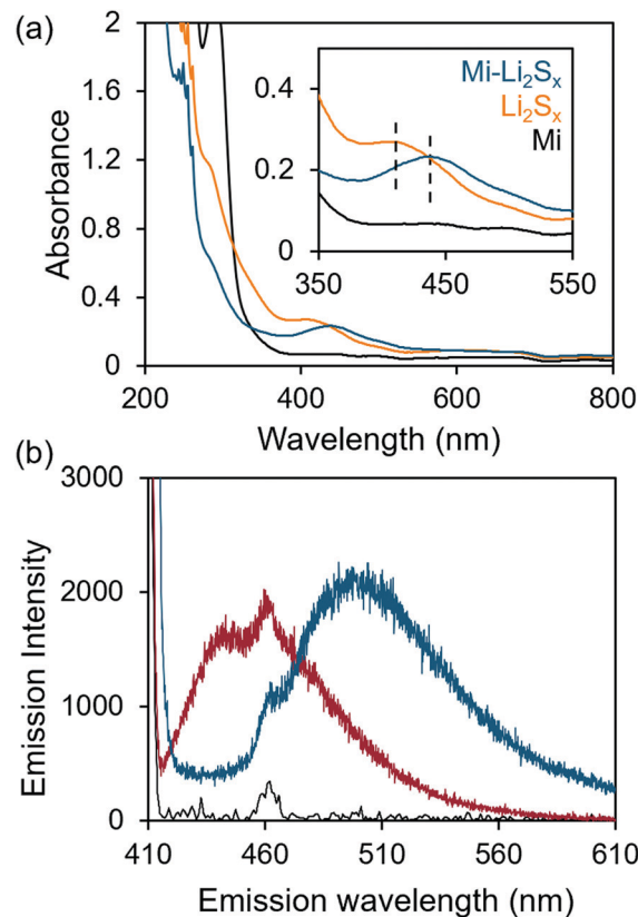
Fig. 1 (a) UV-Vis absorption spectra solutions of Li 2 S x (orange), Mi-BDOME (Mi, black), and Li 2 S x + Mi-BDOME (Mi-Li 2 S x , blue) in 1 : 1 DOL/DME. The inset shows the absorbance change upon addition of Mi-BDOME to Li 2 S x . (b) Fluorescence emission spectra of Mi-BDOME (red) and the Mi-BDOME-Li 2 S x (blue) solutions excited with 405 nm light. The background fluorescence of the solvent mixture is shown in black.
