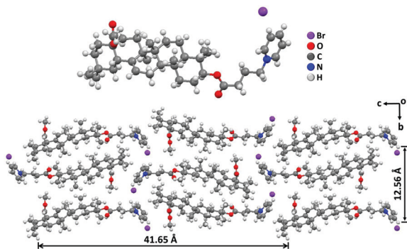
Fig. 3 X-ray single crystal structure of C4-MOP and its spatial arrangements along the directions b and c . Purple: bromine atom, red: oxygen atom, grey: carbon atom, blue: nitrogen atom, white: hydrogen atom.
