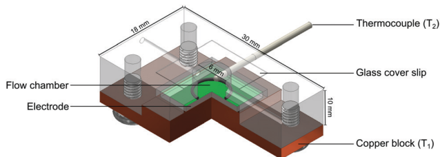
Fig. 3 Schematic of the 3D printed flow cell used for fluorescence and thermal measurements.
