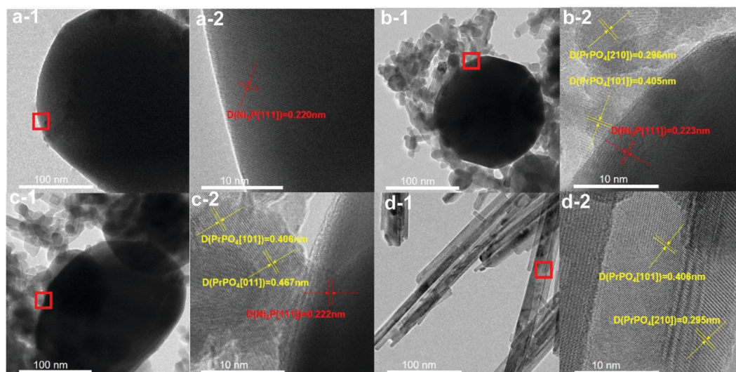
Fig. 2 Typical TEM ( \times - 1 ) and HRTEM ( \times - 2 ) images of samples ( x = a, b, c, and d ). (a) Ni 2 P; (b and c) Pr–Ni–P samples with different Pr: Ni molar ratio (b. Pr: Ni = 0.12; c. Pr: Ni = 0.95); (d) PrPO 4 .
